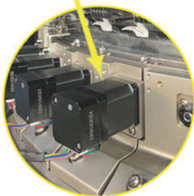
上下盘带自动密度电机 AUTO MATIC STITCH CONTROL BY SERVO MOTOR
